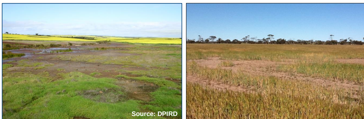
Figure 3. Impact of dryland salinity on agricultural land in the South West – left photo: bare earth salt scalds; right photo: impact of salinity on a cereal crop
