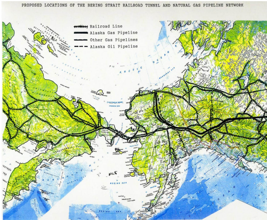
Proposed locations of a Bering Strait Tunnel. Credit: Presented by Hal B. H. Cooper, Jr., President Cooper Consulting Company
