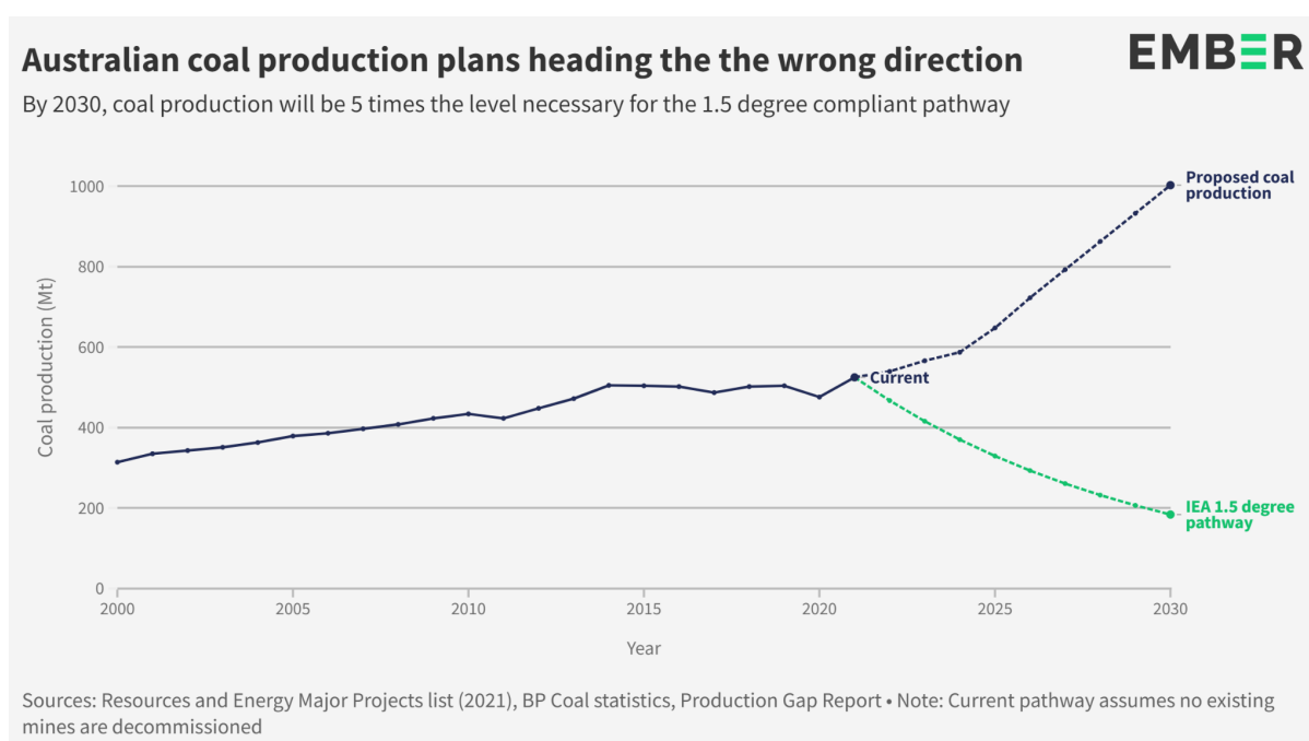
Figure 5: By 2030, Australian coal production will be 5 times larger than the amount needed to achieve a 1.5° compliant pathway in 2030
