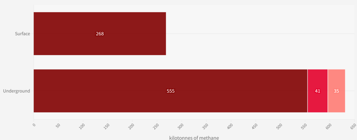
Figure 3: Sources of Australian CMM as reported to AGEIS (2019)
