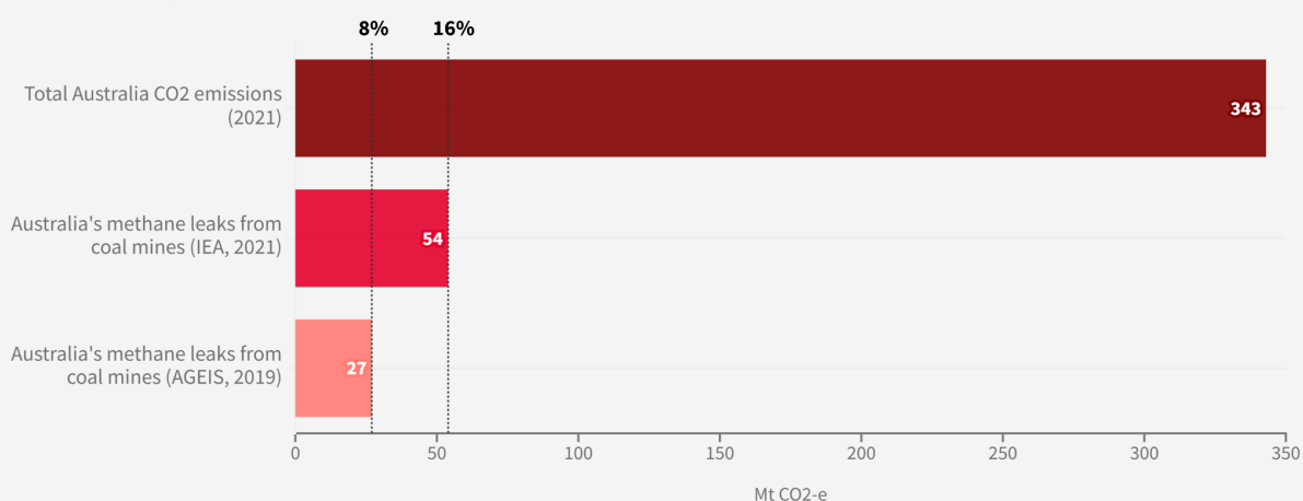
Figure 4: The IEA estimates Australia's coal mines emit twice the amount of methane they officially report, adding 16% on top of Australia's direct CO 2 emissions.
