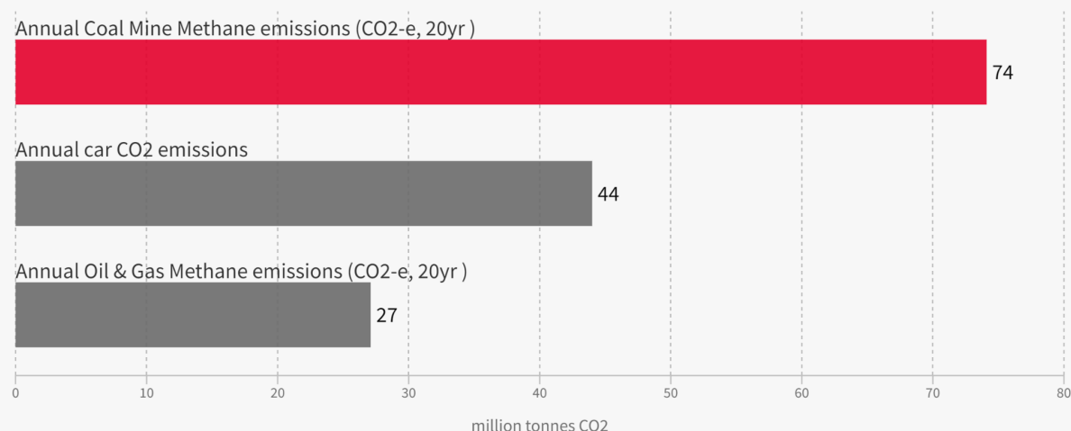
Figure 2: Australian coal mine methane emissions have a short term climate impact of 74 million tonnes of CO 2 .
