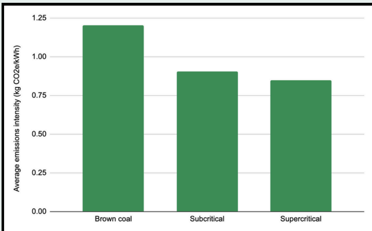
Figure 5: Emissions intensity of brown coal, subcritical black and supercritical black coal-fired power stations in Qld, NSW and Victoria [8].
